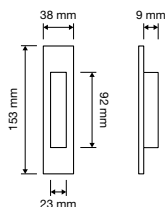
Aida 1611 IP Placca incasso su placca Small / Flush pull on plate Small
