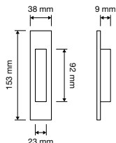
Aisha 1650 IP Placca incasso su placca Small / Flush pull on plate Small
