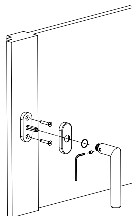
Montaggio maniglia per finestra DK 4-8-scatti / Handle fitting for tilt windows 4-8-clicks
