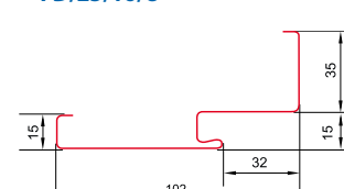
FD/25/16/U
