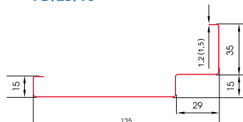
FD/25/16
