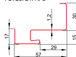
FD/25/21/N/O
